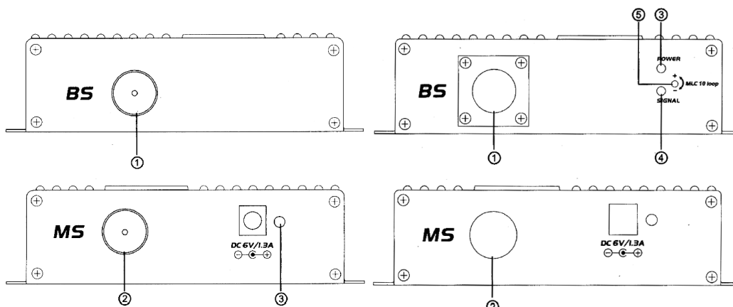
AT-500
